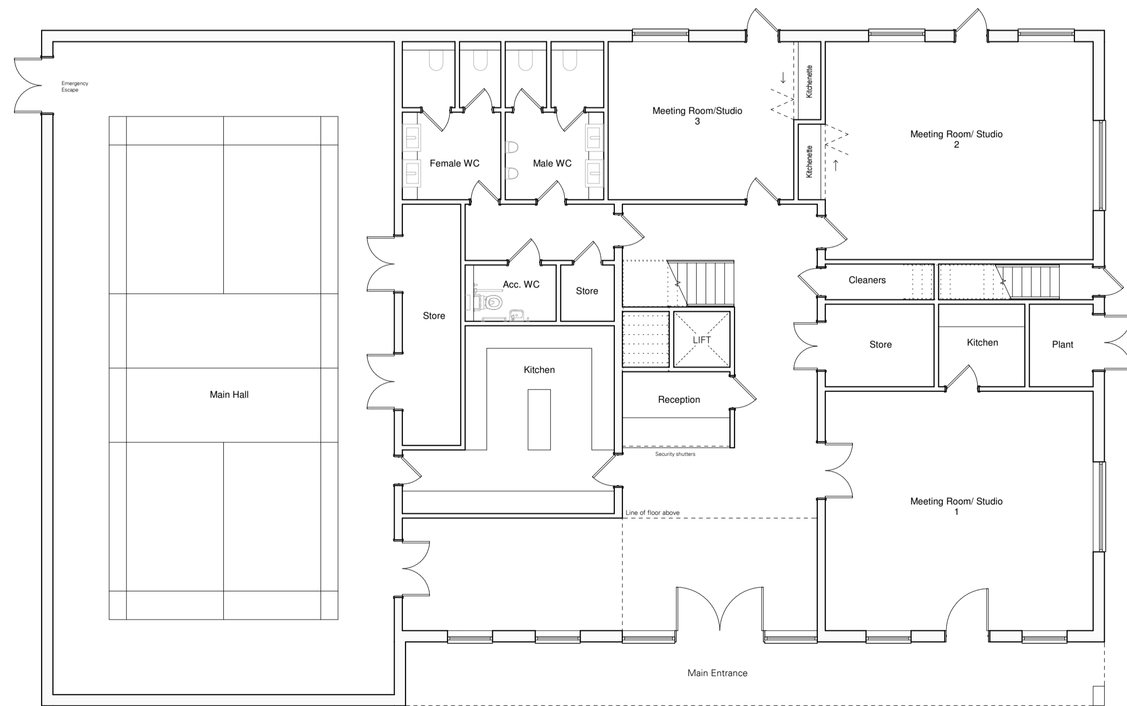
Ground Floor
