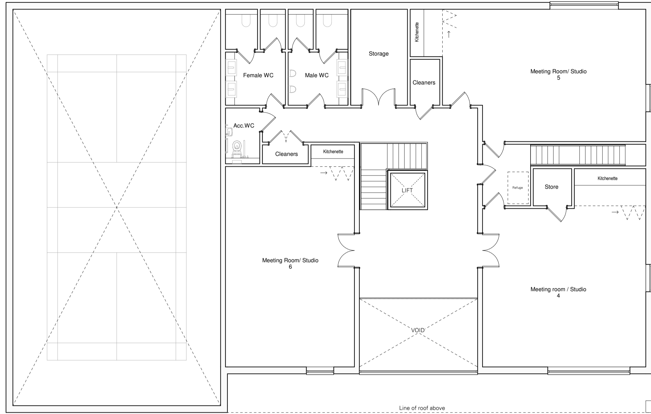
First Floor
